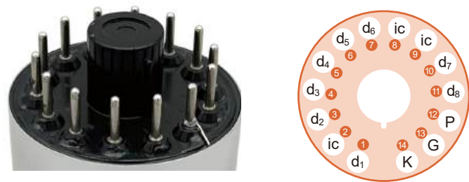
14-pins JEDEC connector (standard pin layout)
