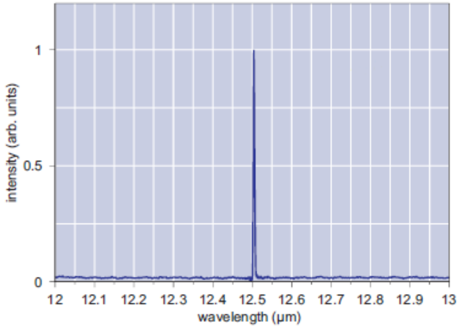
Room Temperature Spectrum at 12.5 \mu\text{m}
