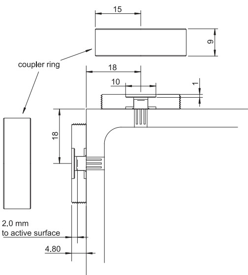
HBPR-200M-30K-SI-FST (1.035"-40 threaded free space input)
