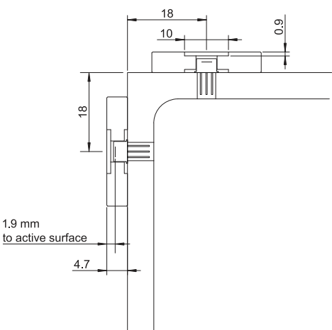
HBPR-200M-30K-SI-FS (25 mm dia. unthreaded free space input)
